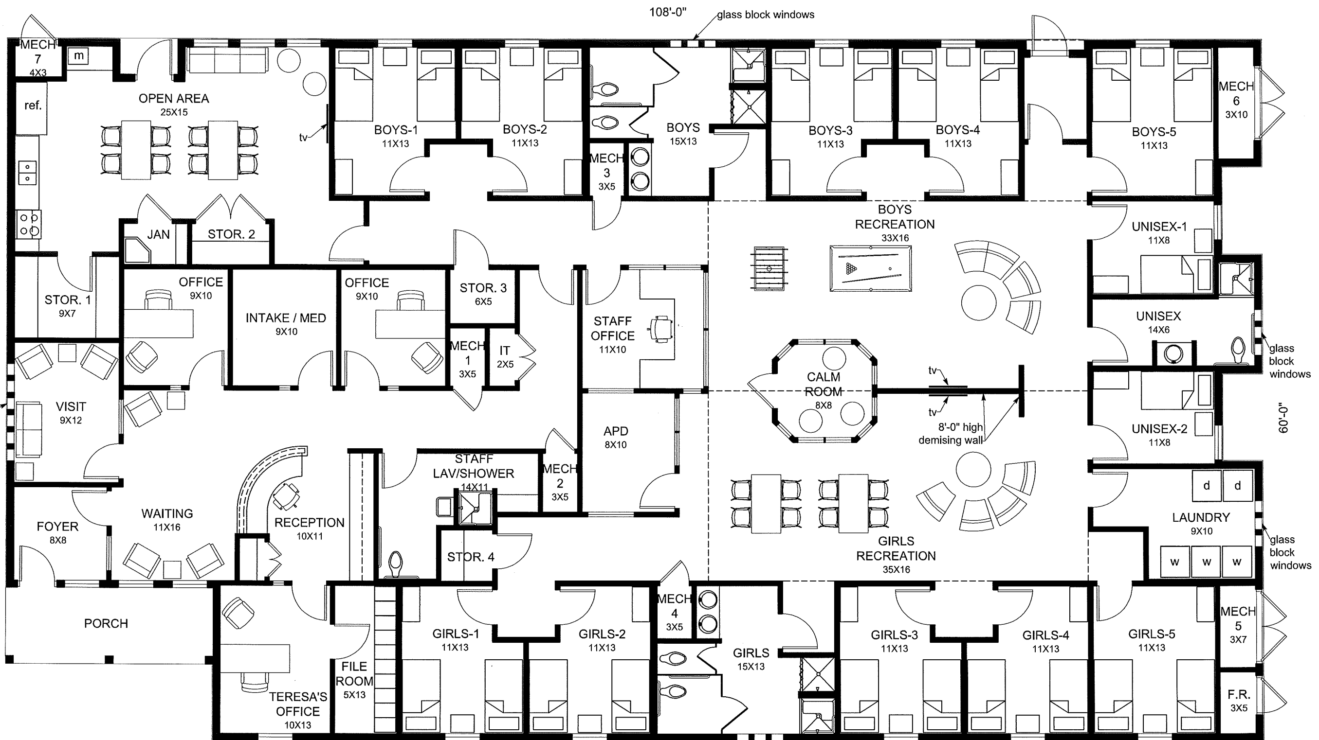
FLOOR PLAN SCALE: 1/8" = 1'-0" 6,480 TOTAL SQ. FT.
